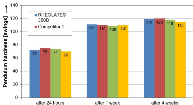
Figure 4: Pendulum hardness
