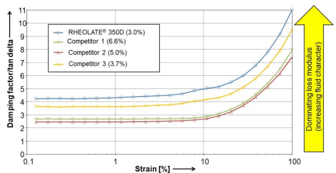
Figure 3: Viscoelasticity
