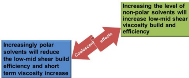
Figure 4: Coalescent influence on HASE efficiency
